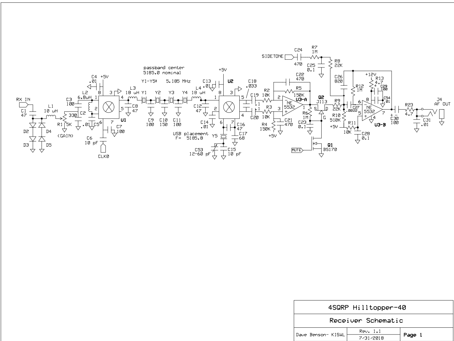
40M Receiver Schematic:
